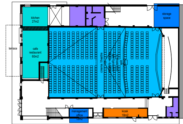
GROUND FLOOR PLAN 480 seats
